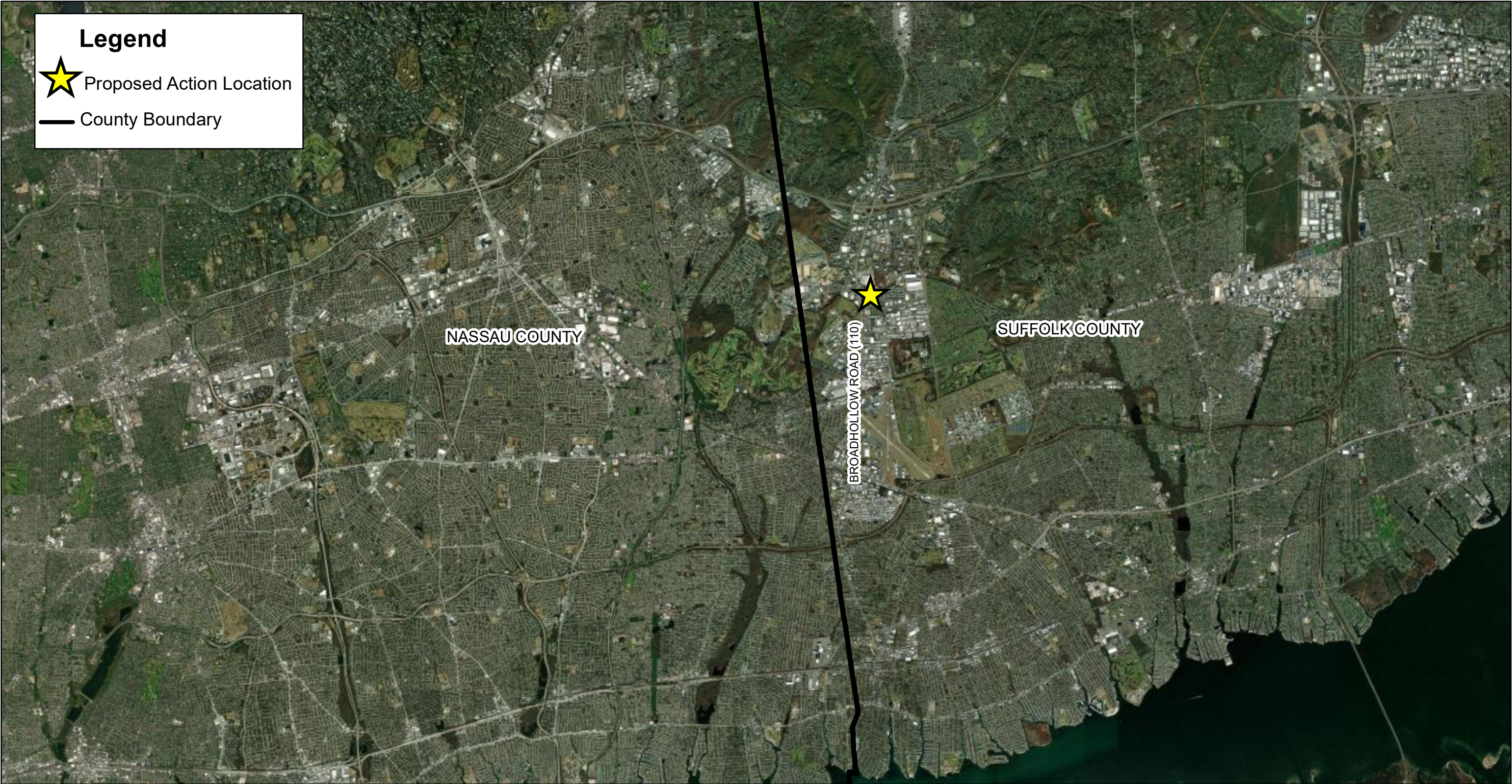
FIGURE 1 RULAND ROAD SUBSTATION EXPANSION AND REACTOR INSTALLATION TOWN OF HUNTINGTON, NEW YORK PROPOSED ACTION LOCATION MAP
