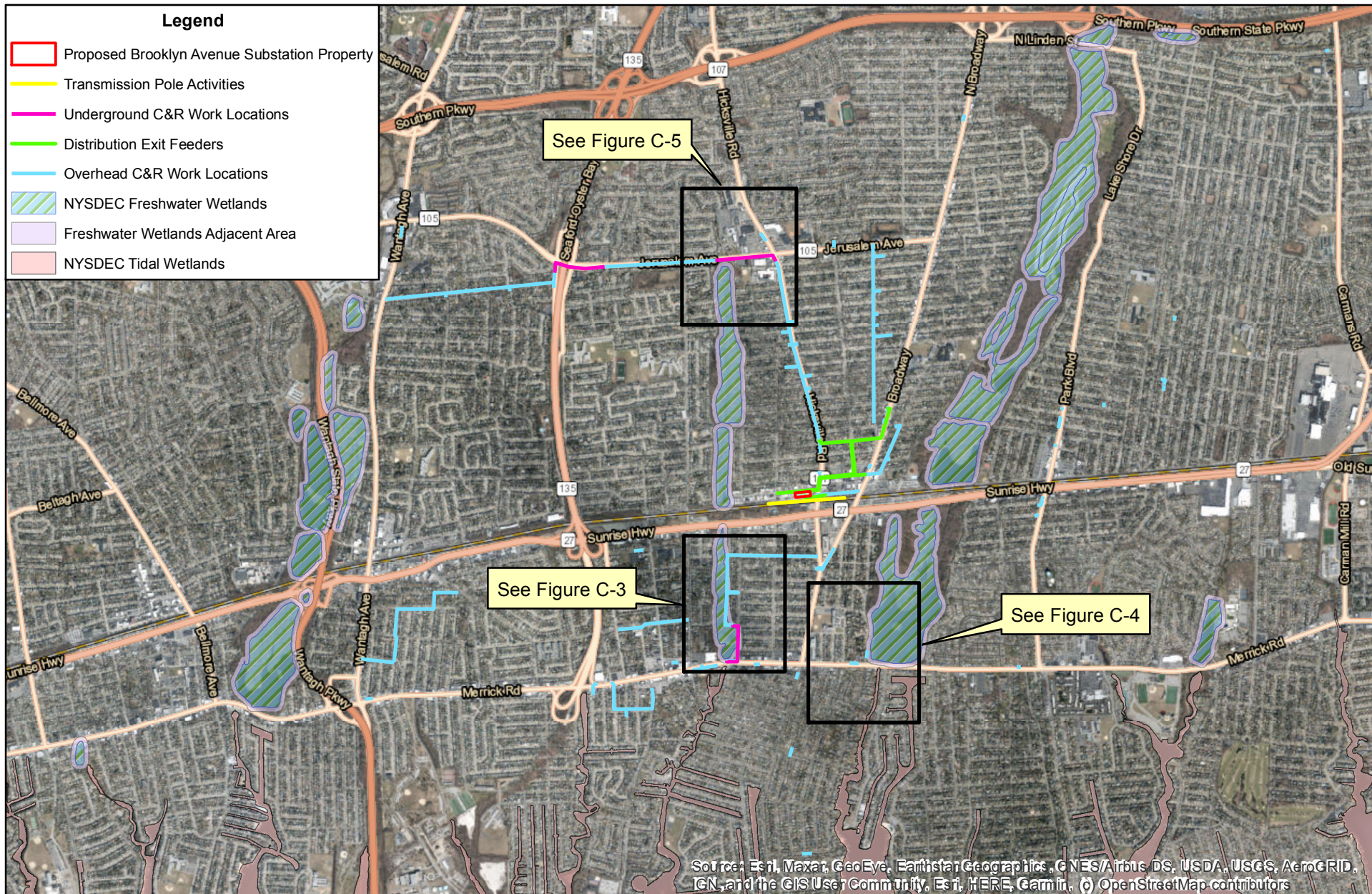
FIGURE C-2 BROOKLYN AVENUE (5BK) NEW SUBSTATION NYSDEC WETLANDS MAP
