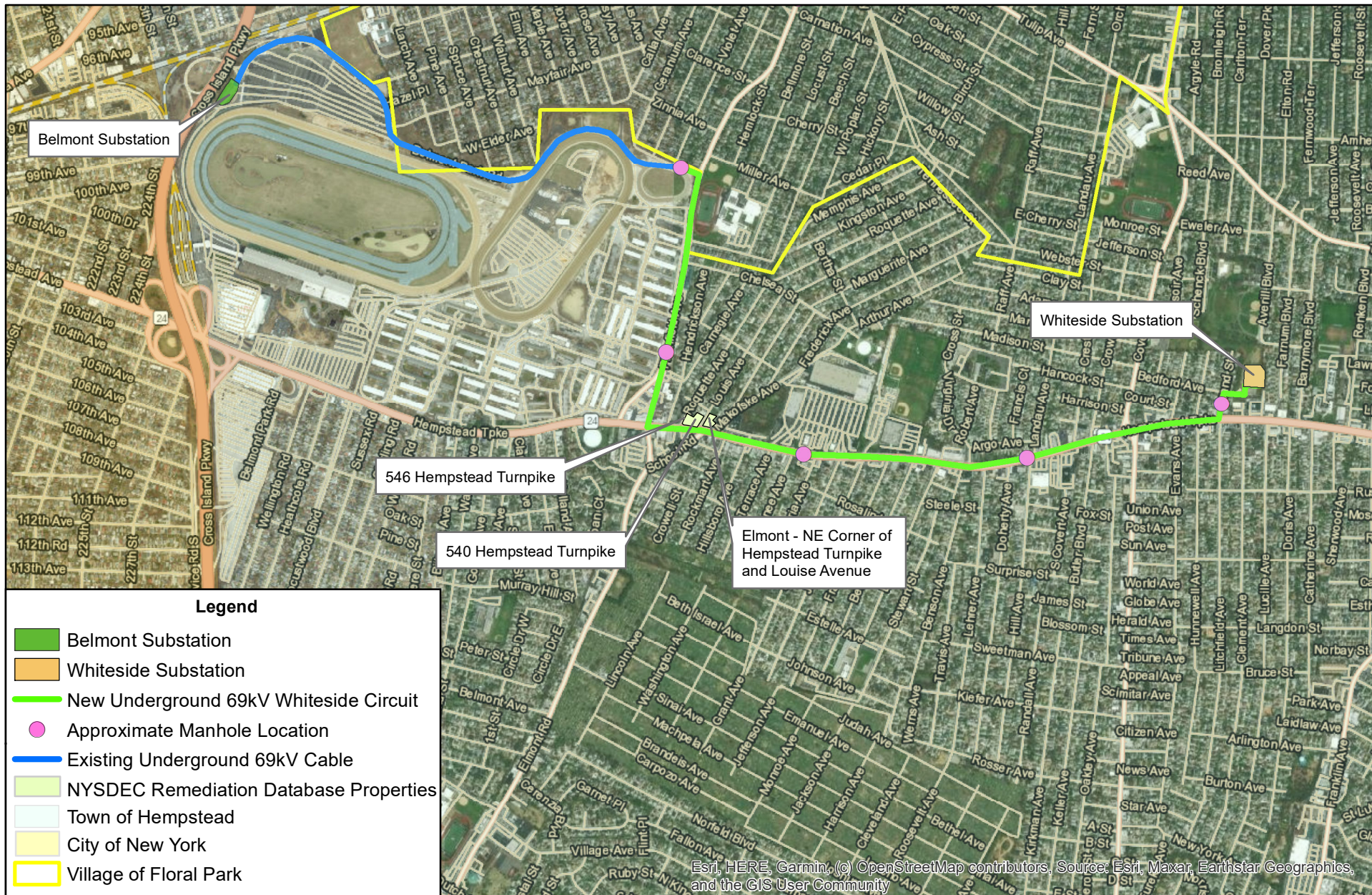
FIGURE 5 BELMONT 69kV CONVERSION & NEW 69kV CIRCUITS TO LAKE SUCCESS AND WHITESIDE WHITESIDE CIRCUIT OVERVIEW MAP
