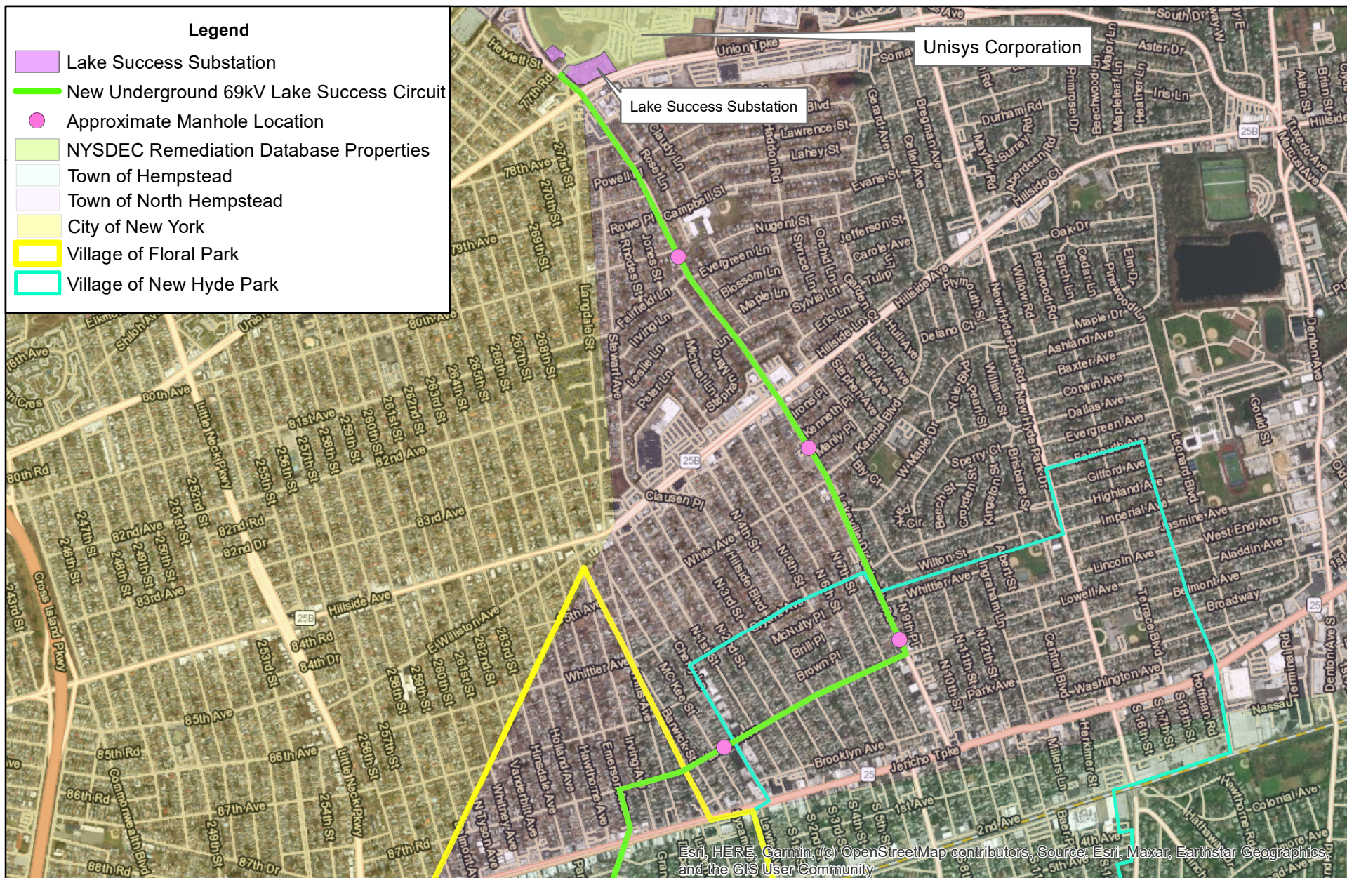
FIGURE 3 BELMONT 69kV CONVERSION & NEW 69kV CIRCUITS TO LAKE SUCCESS AND WHITESIDE LAKE SUCCESS CIRCUIT OVERVIEW MAP
