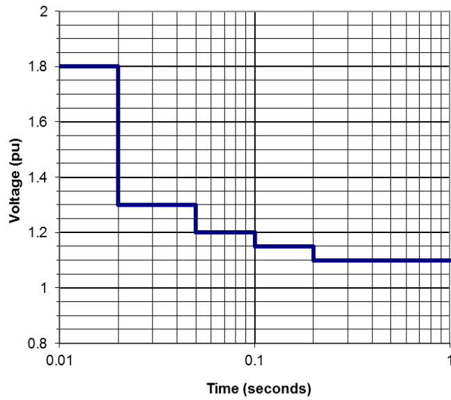
Figure 6-1 Limits to overvoltage caused by Resource
