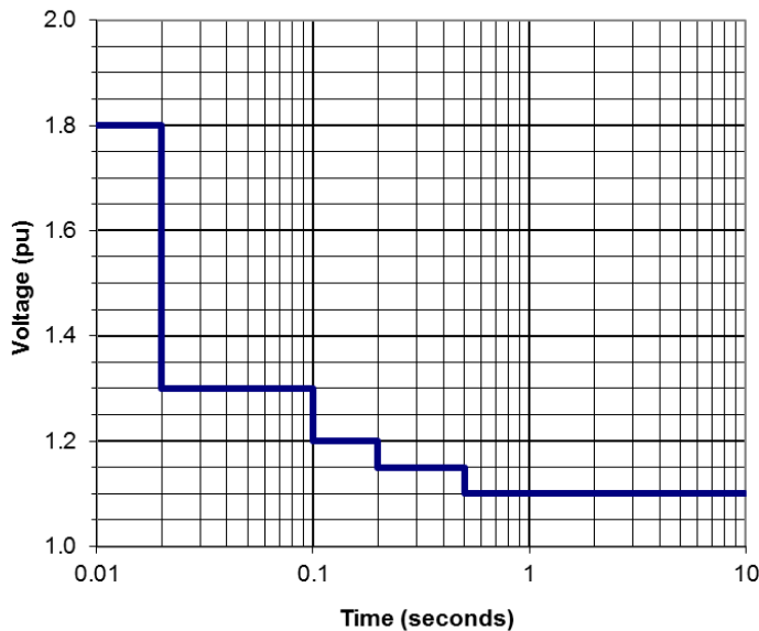
Figure 3-2 Maximum high voltage ride through requirement.
